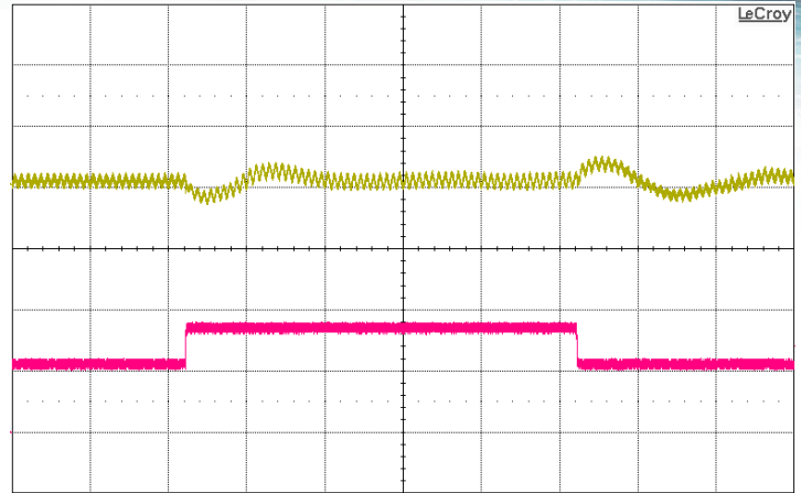
Figure 8: Output voltage response to step-change in load current with 200µF hold-up capacitor (50%-75%-50% of Iout(max), 115Vrms, 60Hz) Top: Vout (2V/div), Bottom: Iout (5A/div), Timebase: (100ms/div).
