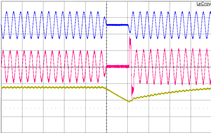
Figure 7: Line drop out with 400µF hold-up capacitor at full load current (115Vrms, 60Hz) Top: Vin (200V/div), Mid: Iin (5A/div), Bottom: Vout (10V/div), Timebase: (50ms/div).
