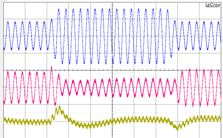
Figure 10: Input voltage transient response with 200µF hold-up capacitor at full load current (115Vrms-230Vrms-115Vrms, 60Hz), Top: Vin (200V/div), Mid: Iin (5A/div), Bottom: Vout (2V/div), Timebase: (50ms/div).
